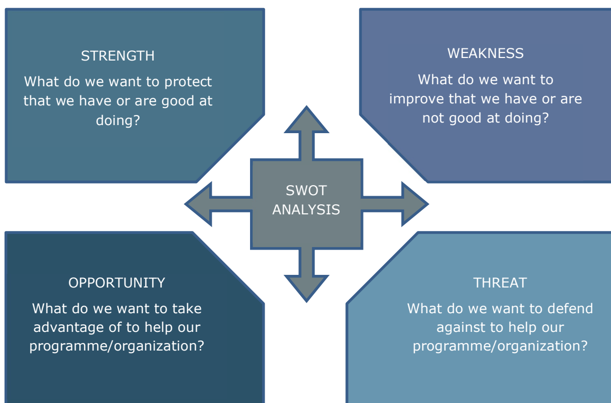
Fig 6. SWOT analysis
